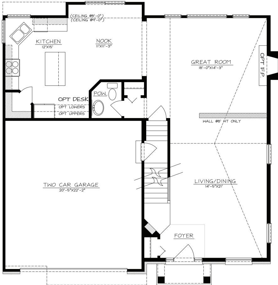
MAIN LEVEL FLOOR PLAN
